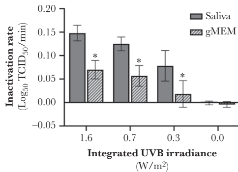
Figure 6. SARS-CoV-2 inactivation rates as a function of UVB level. Inactivation of SARS-CoV-2 on stainless steel coupons was significantly greater in the presence of simulated sunlight than that observed in darkness. The UVB level and the suspension matrix both significantly affected the measured inactivation rate. * P < .05 when compared to saliva at the same UVB irradiance level. Values are best fit slopes from linear regression with associated 95% confidence intervals. Abbreviations: gMEM, growth medium; TCID 50 , median tissue culture infectious dose.
